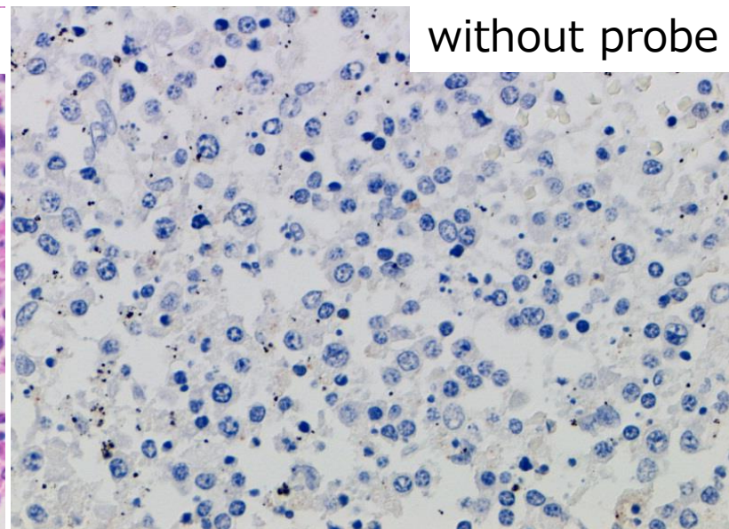
without AT-tailing
